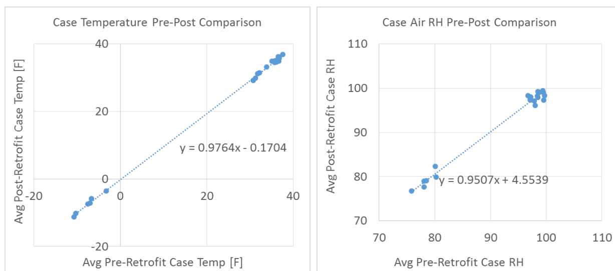
FIGURE 14 – AVERAGE TEMPERATURE AND HUMIDITY COMPARISONS FOR EACH CASE
